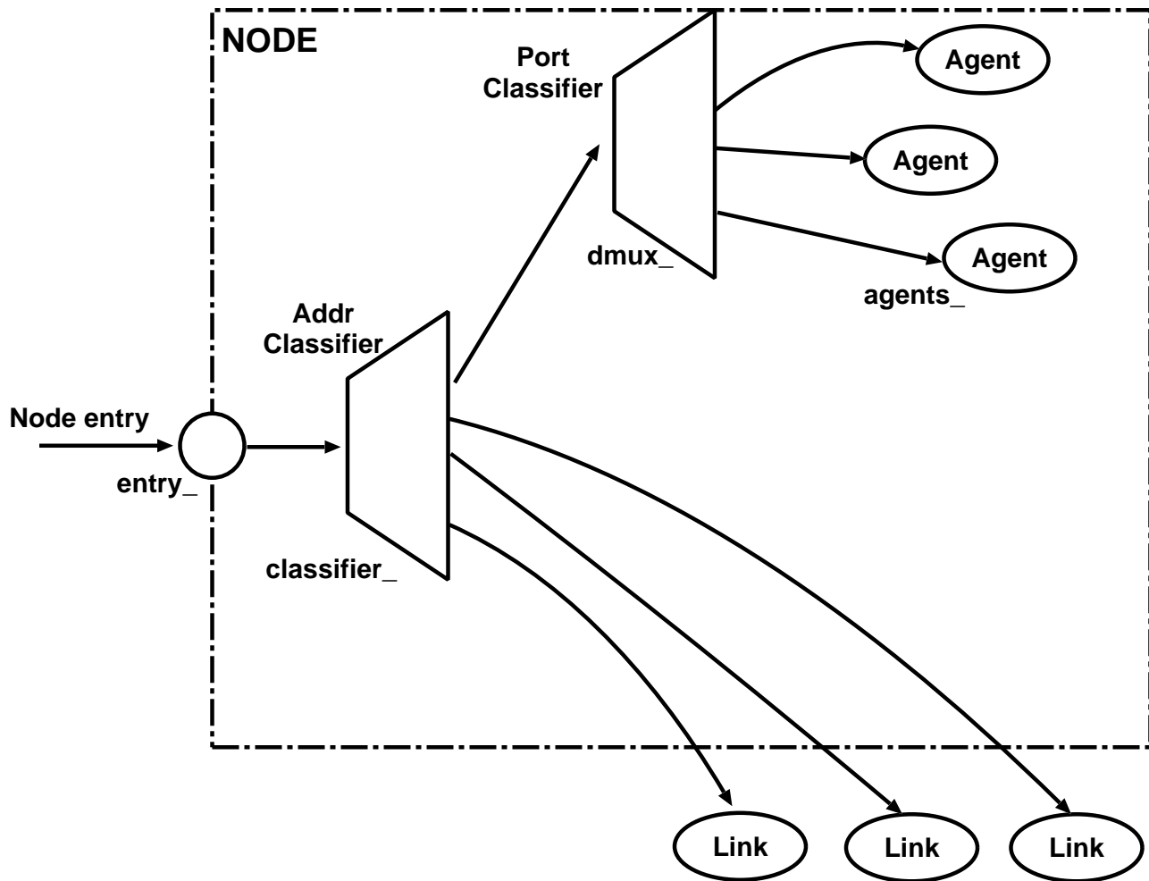
Figure 5.1: Structure of an Unicast Node
