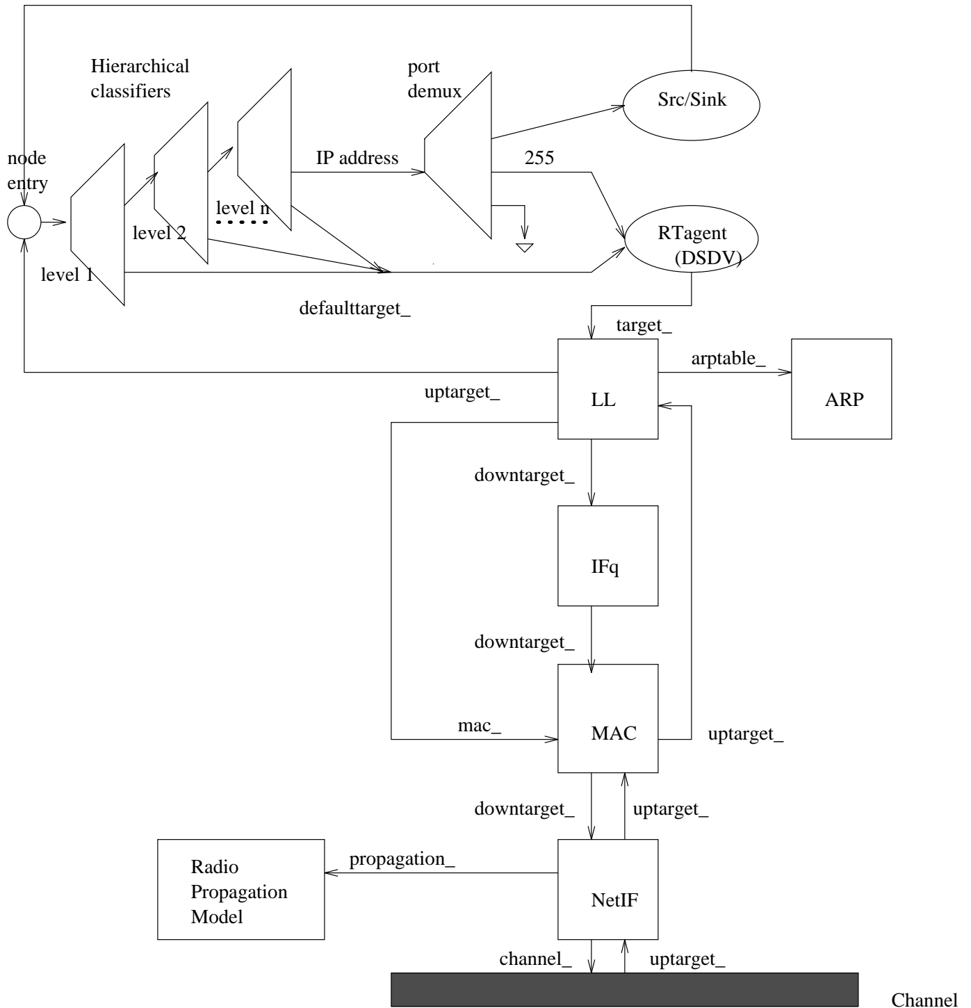
Figure 15.3: Schematic of a baseStationNode
