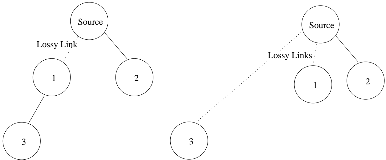
Figure 33.1: Comparison of Multicast Trees for Detailed vs. Session Routing
