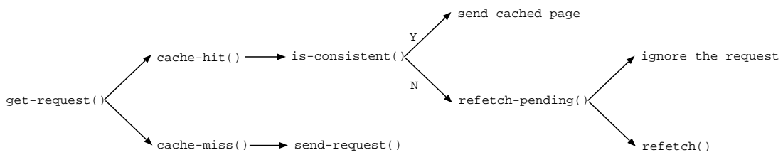
Figure 41.4: Handling of incoming request in Http/Cache
